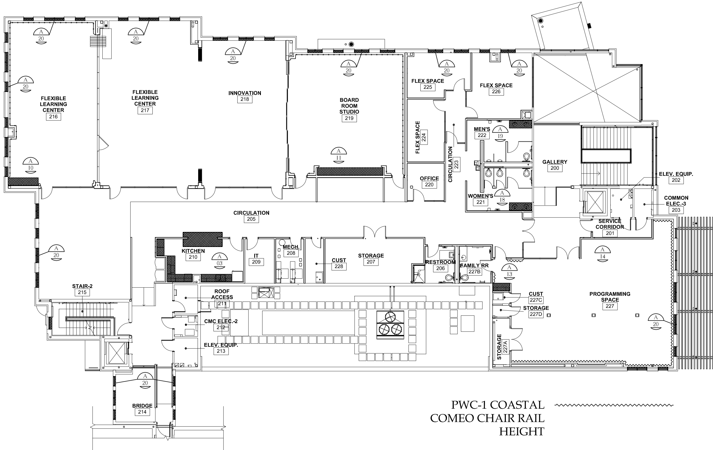
A 02 LEVEL 2 FLOOR PLAN NTS" = 1' ARCH REF: 1/A-102
